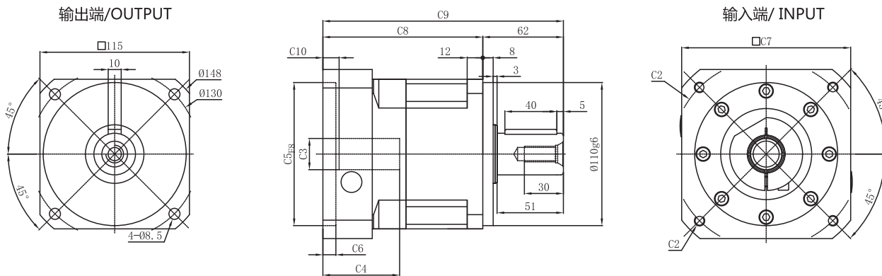
PGL115-L2
