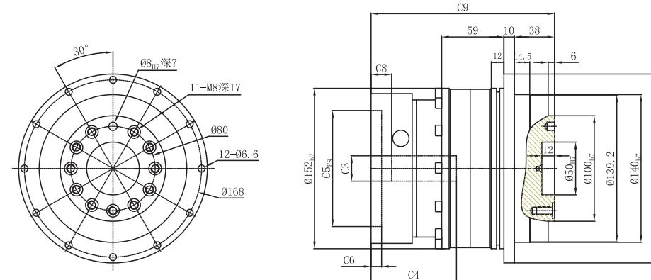
输出端/OUTPUT
