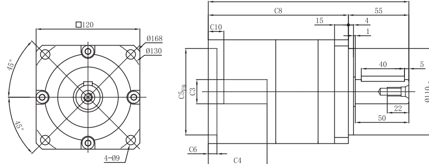
输出端/OUTPUT
