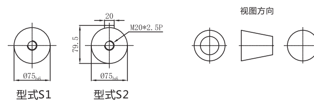
输出轴径/Output Diameter
