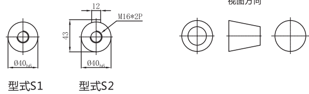
输出轴径/Output Diameter
