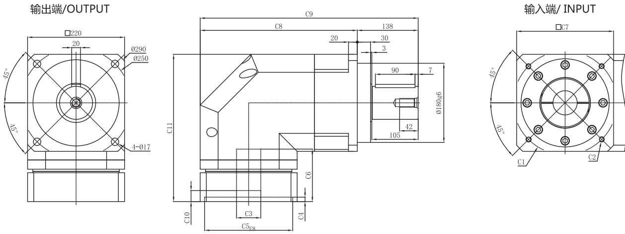
PGHR220-L1
