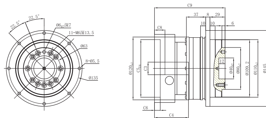
输出端/OUTPUT
