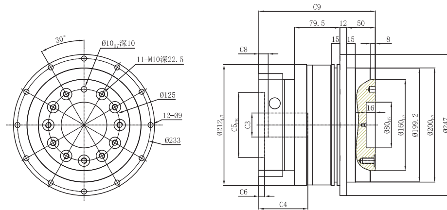
输出端/OUTPUT
