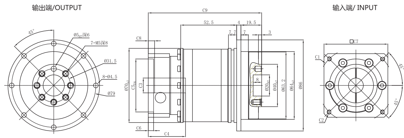
PGF064-L2
