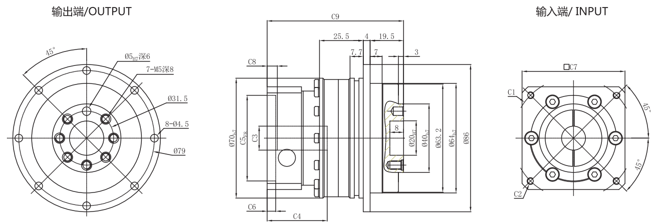
PGF064-L1
