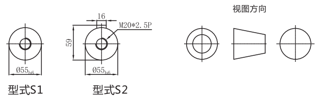
输出轴径/Output Diameter
