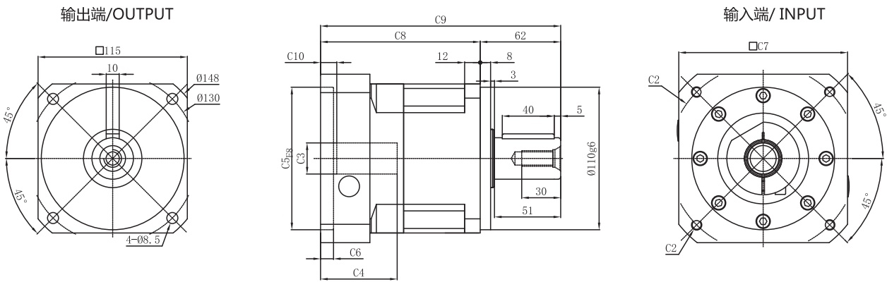
PGH115-L2
