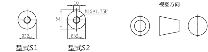
输出轴径/Output Diameter
