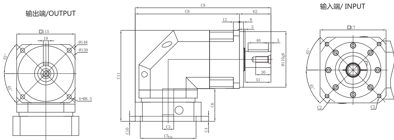
PGHR115-L1
