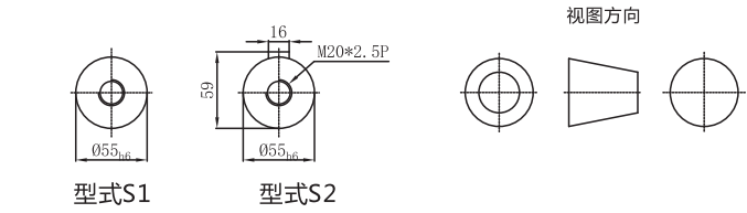
输出轴径/Output Diameter
