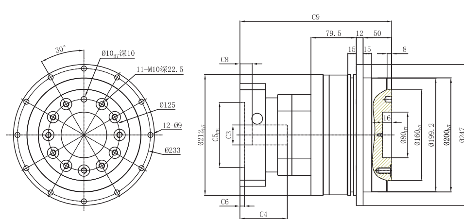
输出端/OUTPUT
