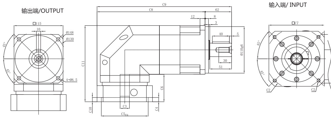
PGHR115-L2
