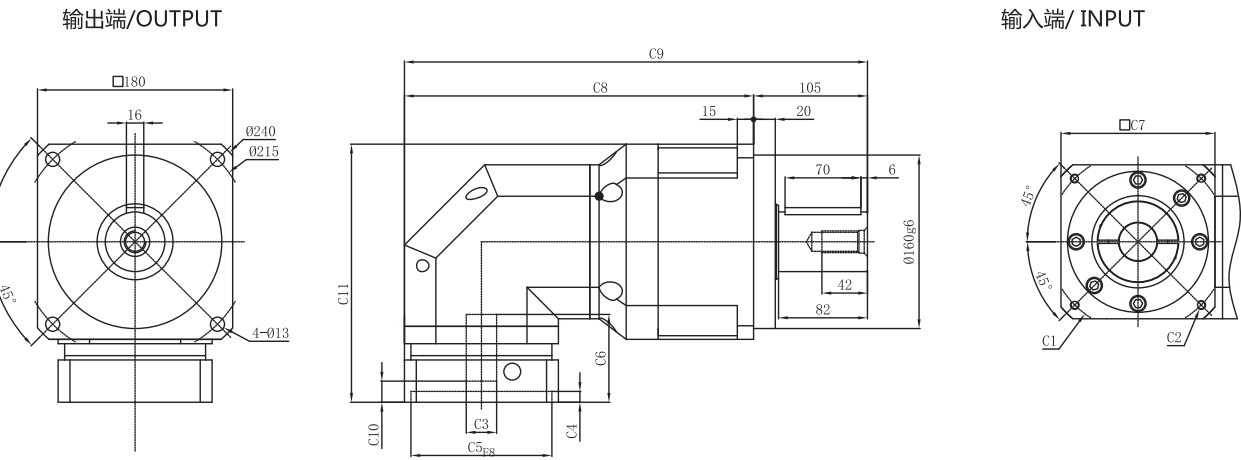
PGHR180-L2
