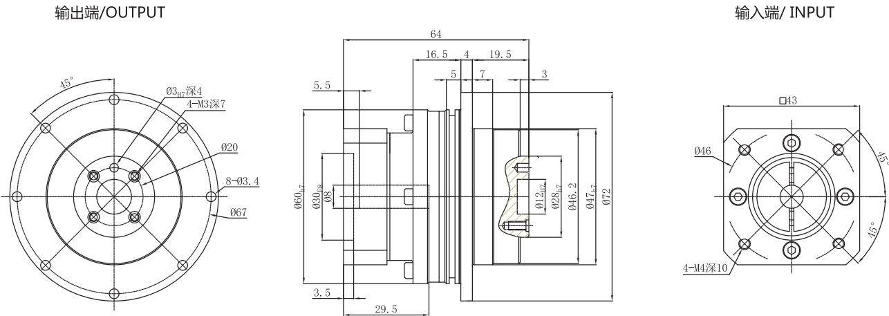
PGF 047-L1
